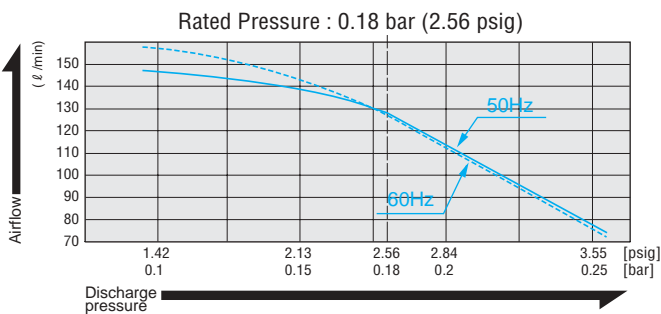
Liquid Mixer Bubbling
